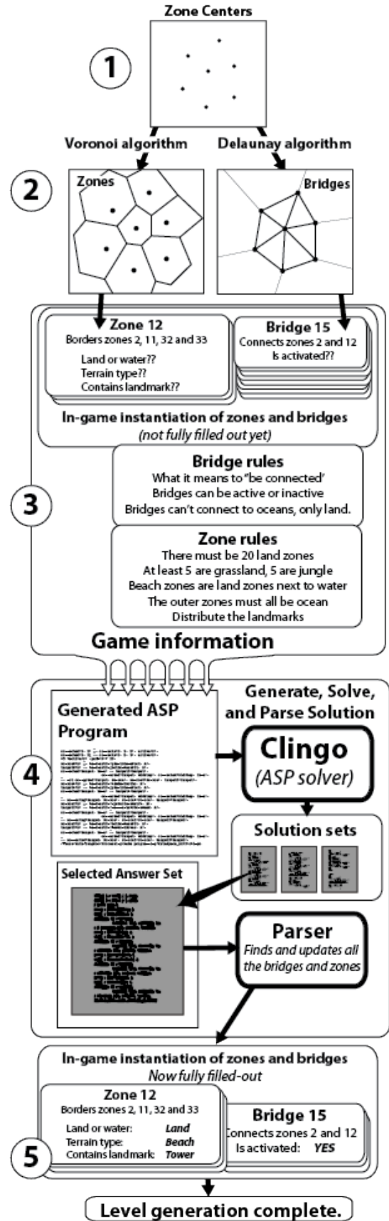
Figure 4: ASP for replayability, generating a level
