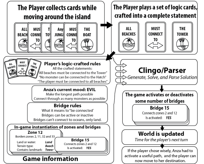
Figure 3: Adaptive PCG with ASP: the prototype responds to a player's crafted logic statement.
